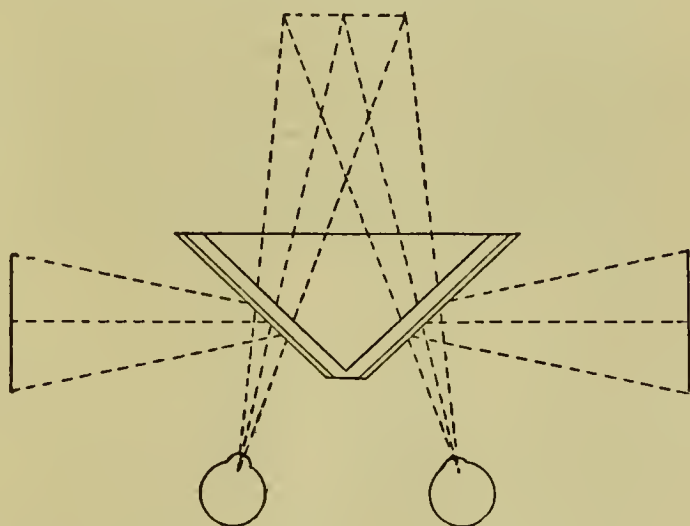
FIG. 49. Plan of Wheatstone's Stereoscope.
